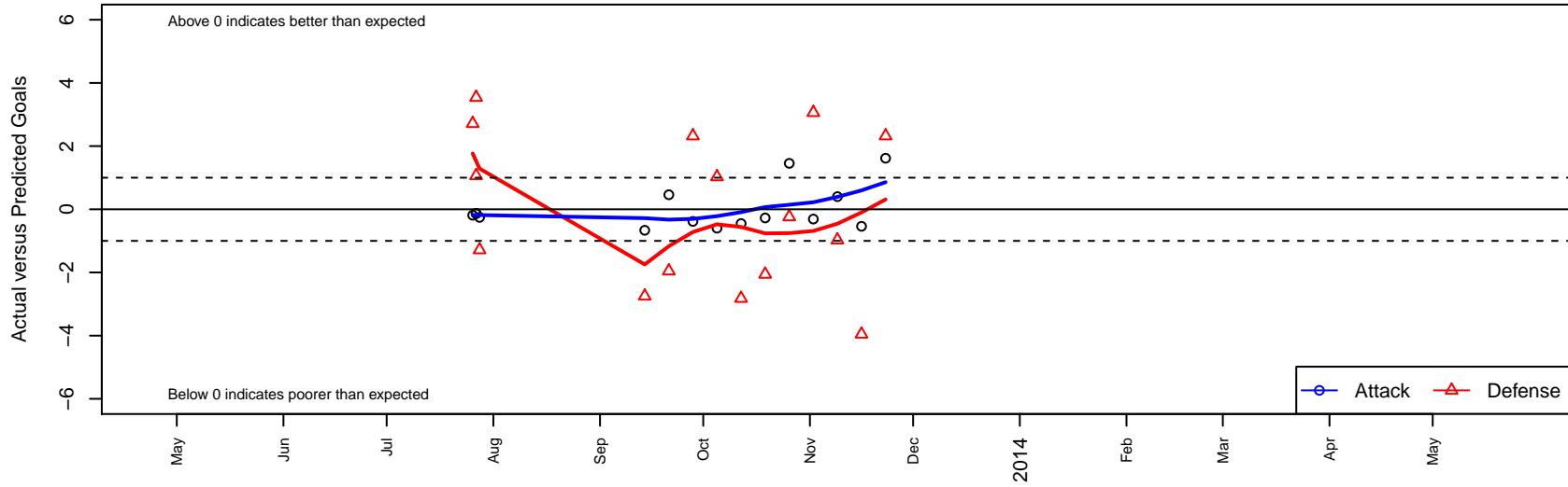
MIFC Grizzlies G01 Dots are actual minus expected GF (blue circles) and GA (red triangles). Blue line is smoothed change in attack strength. Red is smoothed change in defense strength.
